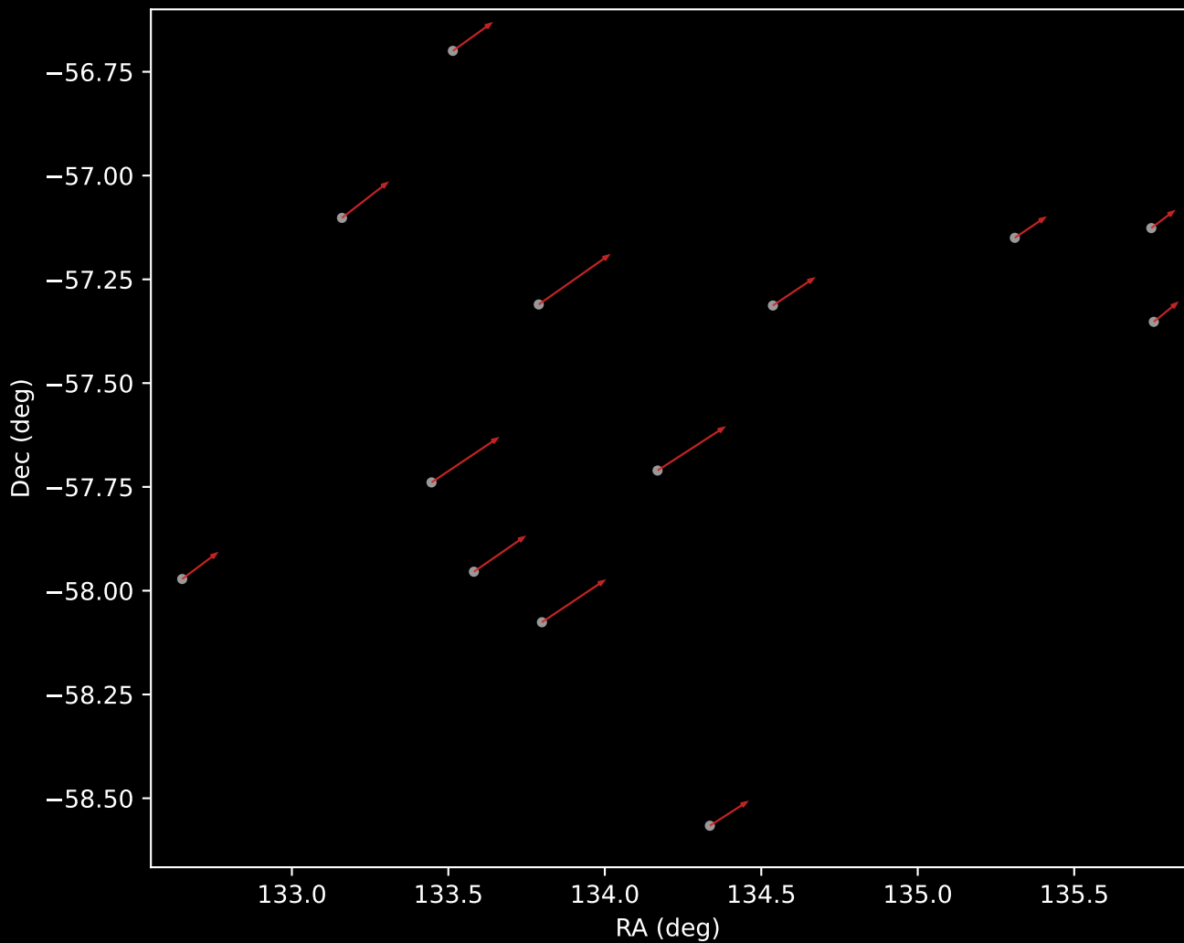
GALAH DR4 Cluster 6 Proper Motion Vectors (n=13)
