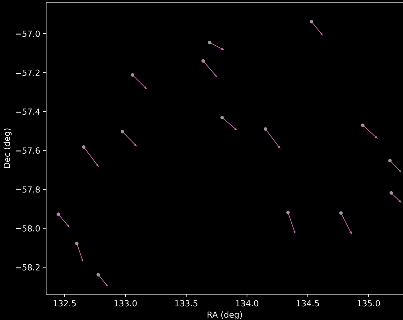
GALAH DR4 Cluster 12 Proper Motion Vectors (n=16)
