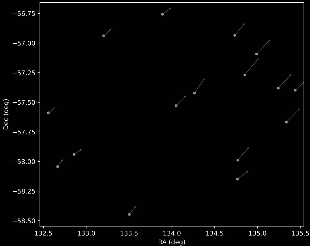
GALAH DR4 Cluster 10 Proper Motion Vectors (n=16)
