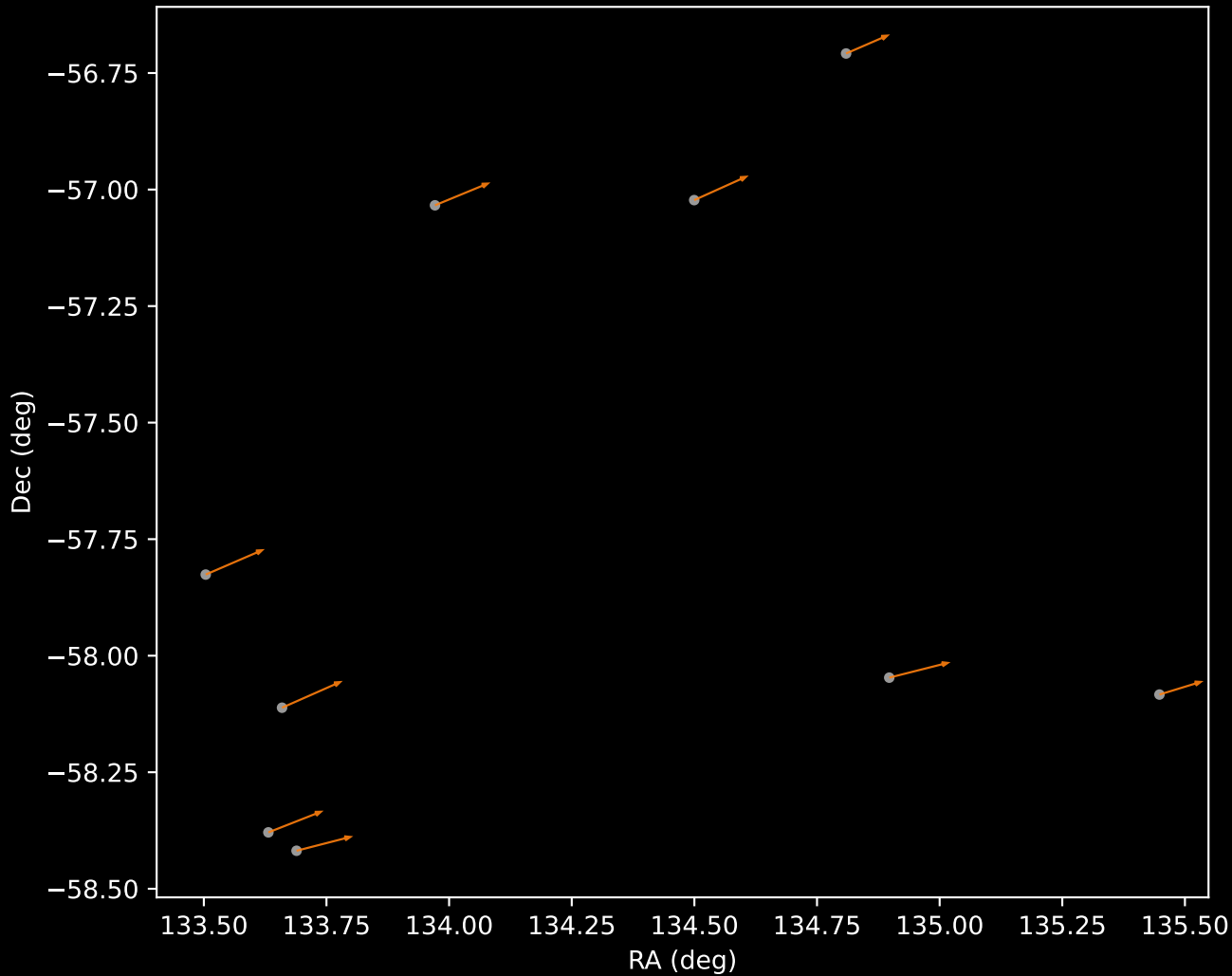
GALAH DR4 Cluster 2 Proper Motion Vectors (n=9)
