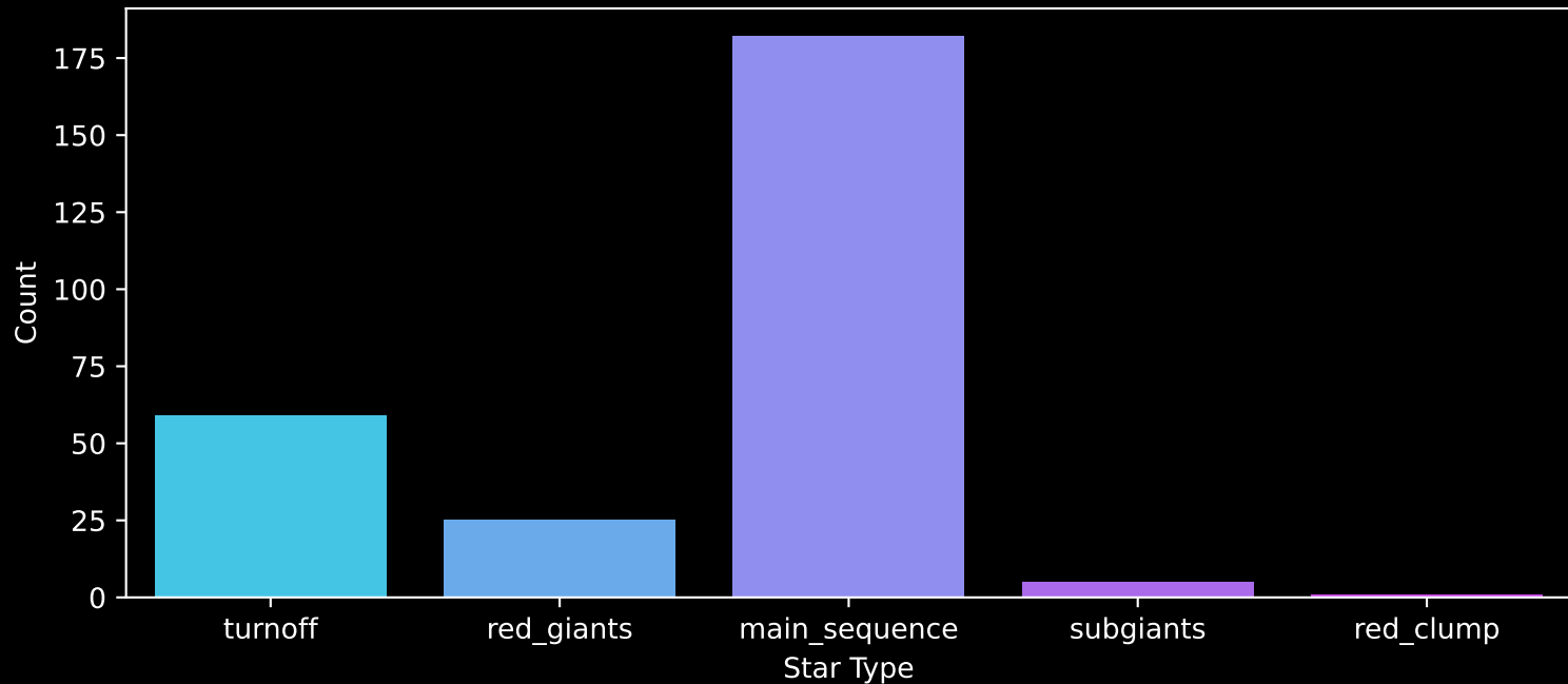
GALAH DR4 Field: [6886] Count plot of Star Type
