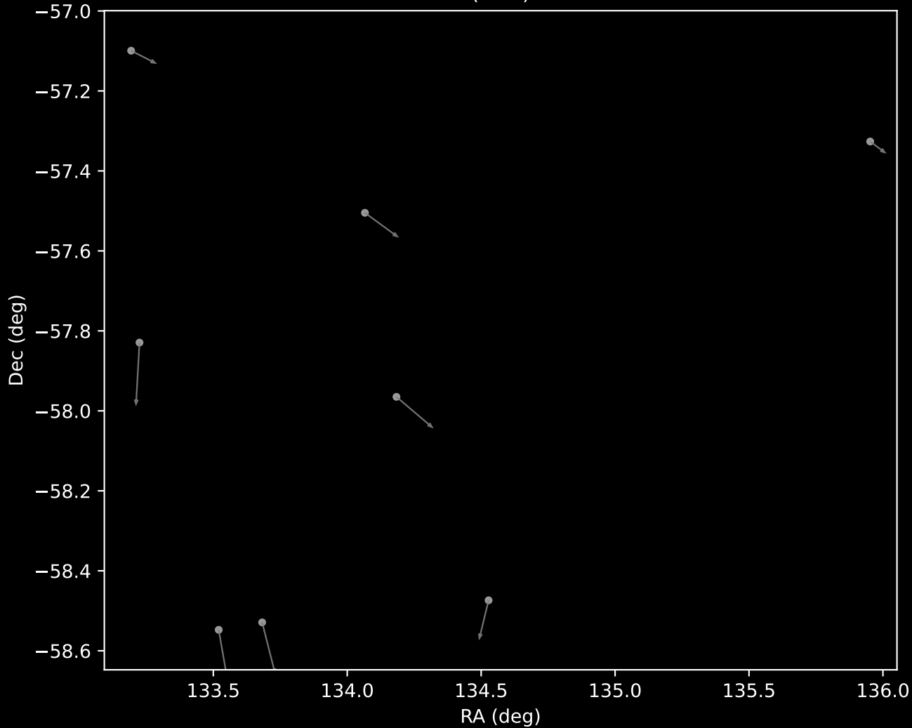
GALAH DR4 Cluster 14 Proper Motion Vectors (n=8)
