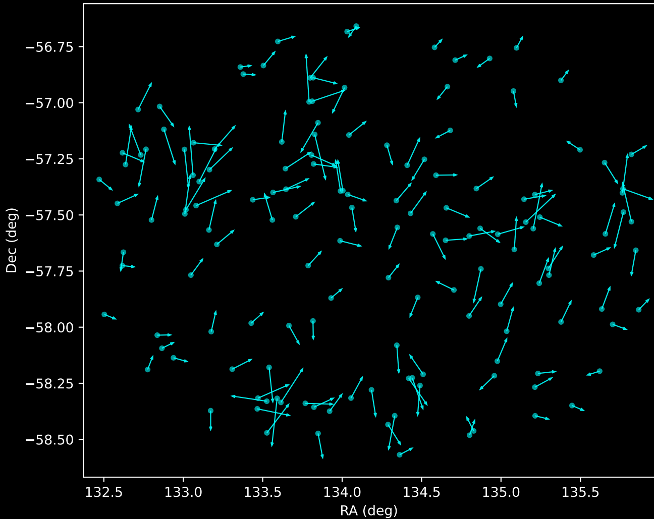
GALAH DR4 Noise Stream Proper Motion Vectors (n=147)
