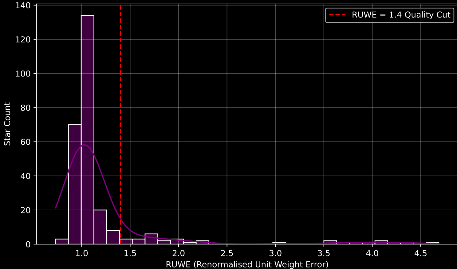
GALAH DR4 Field [6886] RUWE Distribution (n= 265)
